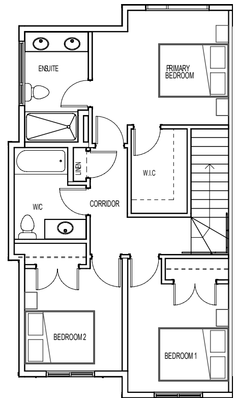
THIRD FLOOR
